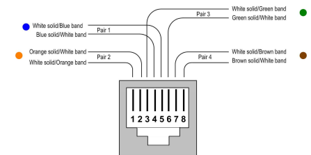
RJ45 Jack EIA/TIA 568B
